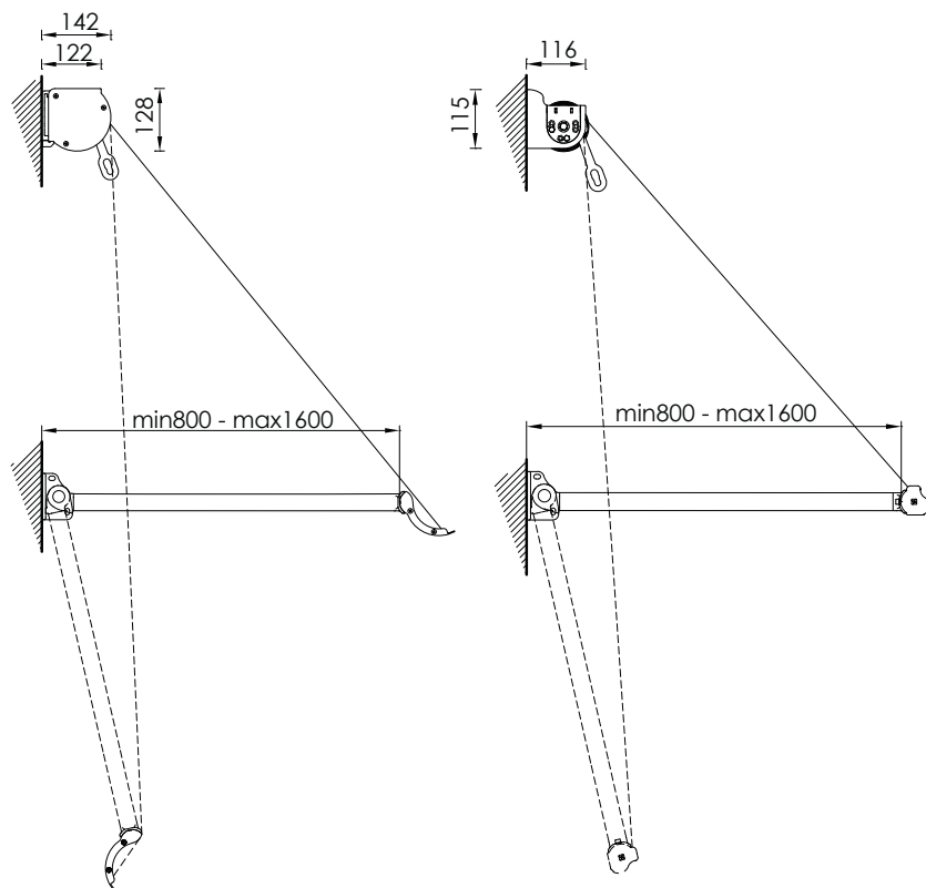
Montaggio a parete Wall installation
