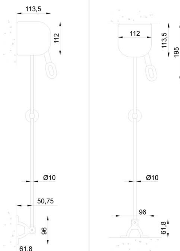
Montaggio a parete Wall installation
