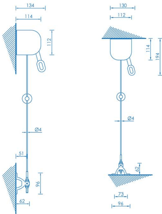
Montaggio a parete Wall installation
