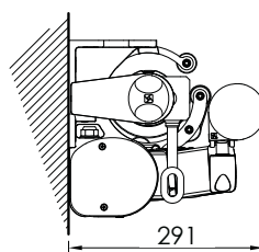
Montaggio a parete Wall installation
